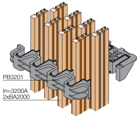
Example of use of 2 busbars per phase (3200A)
