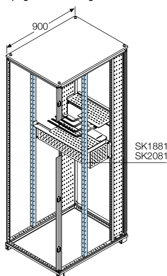
Uprights for switchgear D=900mm
