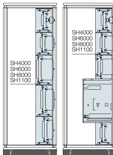
Example of Form 3a segregation
