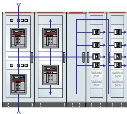
ArTu K Series dim. 1800x2280x700 (2031x2900x837) mm (external hwxwd) IP65 with Emax E2, T5, T3, XT3 3200A omnibus busbars and vertical 1600A branches - Icw 65kA
