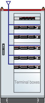
ArTu M Series dim. 1600x800x250 (1796x924x250) mm (external hxwxh) IP65 with modular panels
