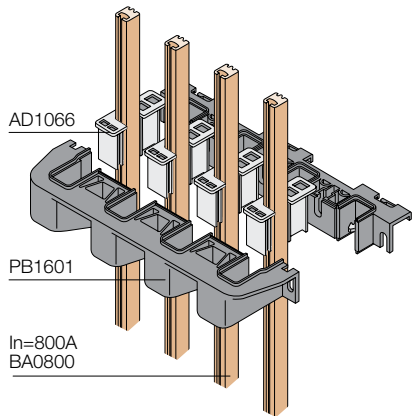
Example of use of adapter for busbars
