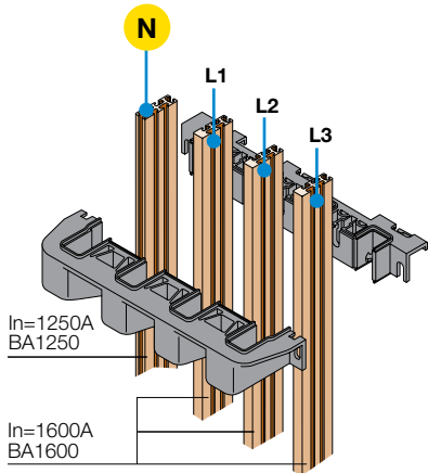
Example of use of the busbar with reduced neutral
