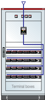
ArTu K Series dim. 1800x800x225 (2031x948x362)mm (external hwxwd) IP65 with plate for Tmax T5 and modular panels
