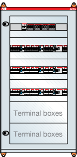
ArTu M Series dim. 1200x600x200 (1300x700x200) mm (external hxwxd) IP65 with modular panels
