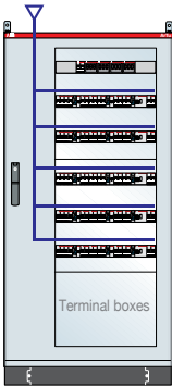
ArTu K Series dim. 1600x800x150 (1831x948x287) mm (external hxwx d) IP65 with modular panels
